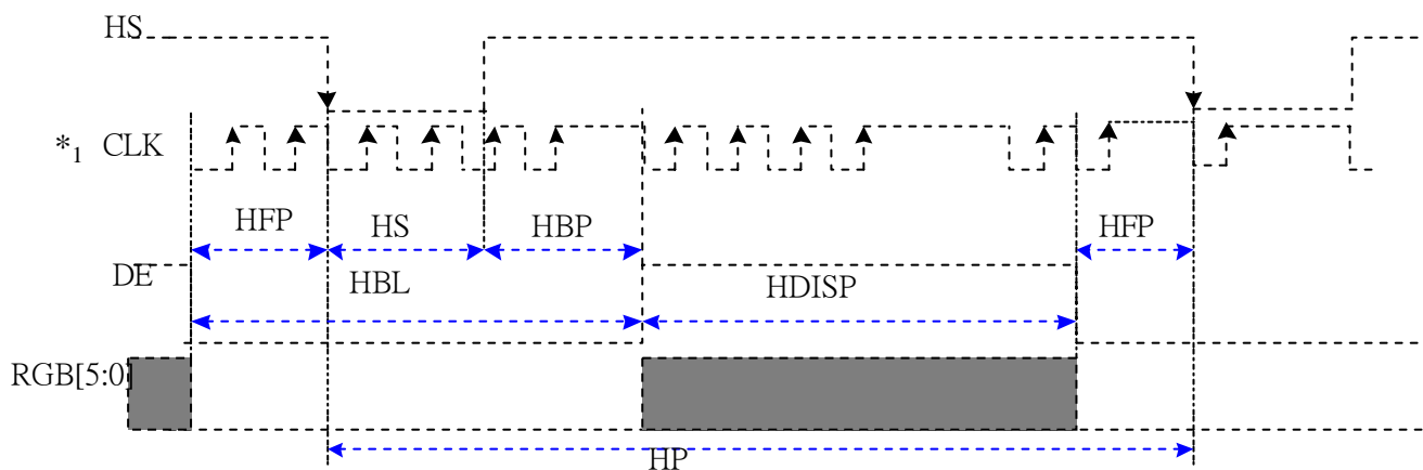
< Horizontal Timing chart >
