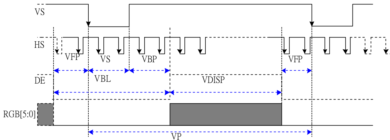
< Vertical Timing chart >
