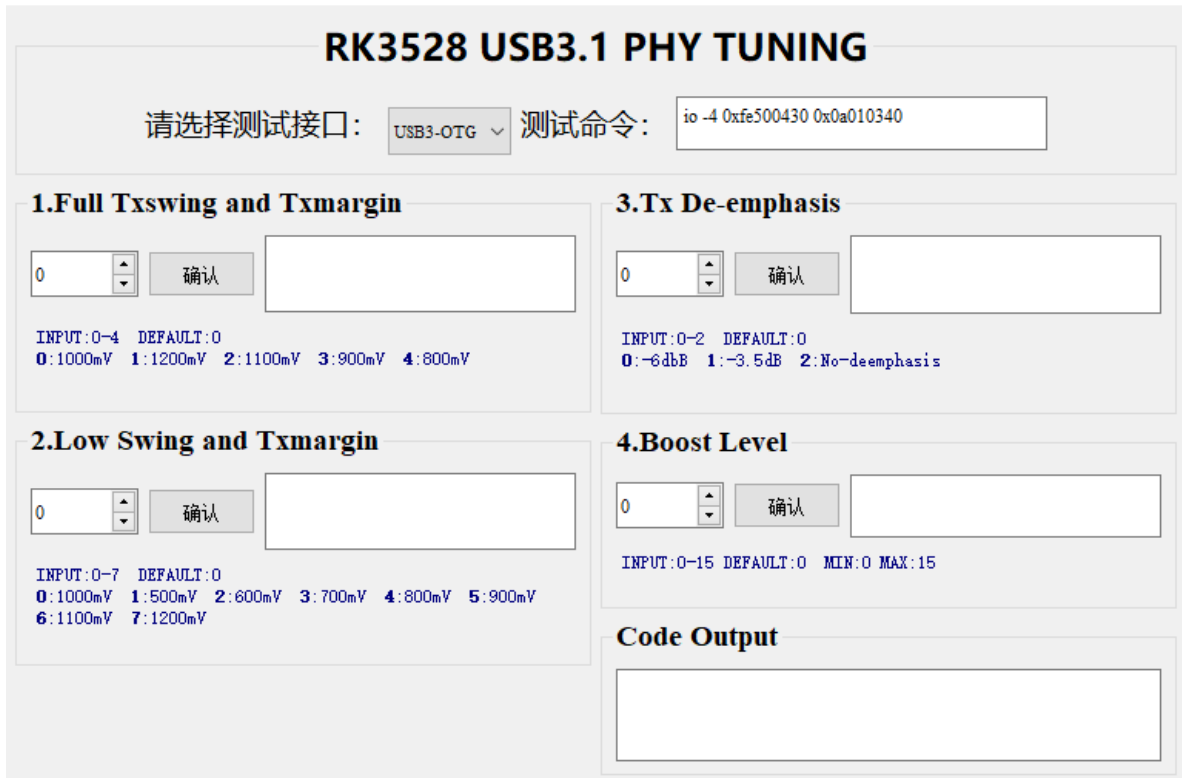
图9 RK3528 USB3.1 PHY Tuning Interface
