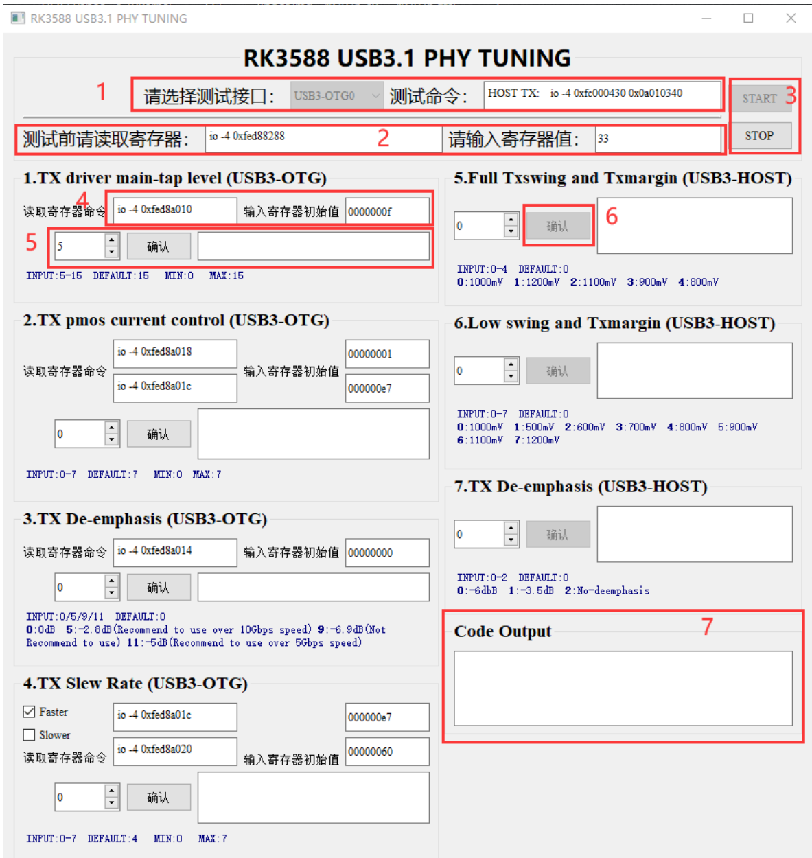
图6 RK3588 USB3.0 PHY Tuning Interface
