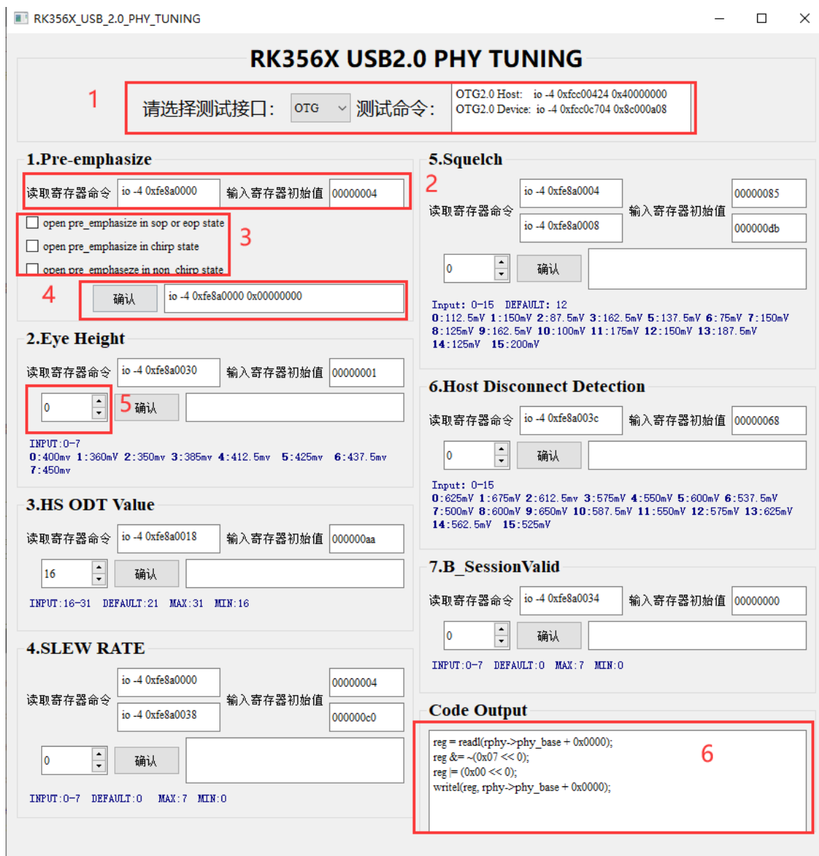
图3 RK3568 USB2.0 PHY Tuning Interface
