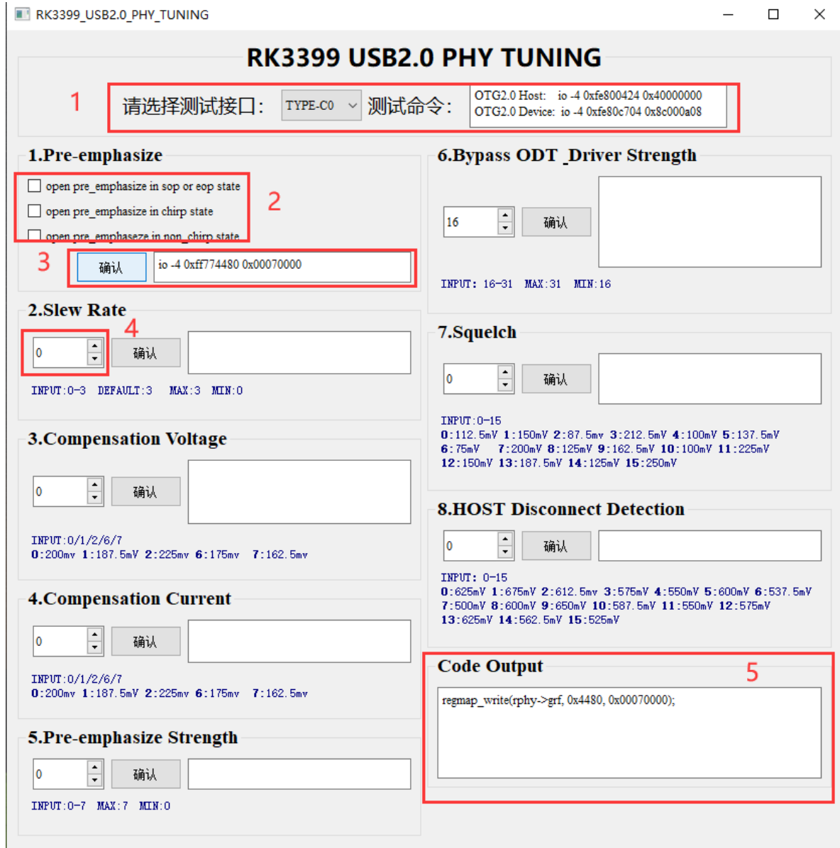
图2 RK3399 USB2.0 PHY Tuning Interface
