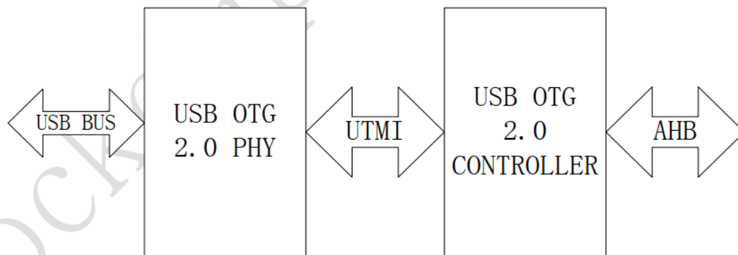
Figure 1-2 USB 2.0 OTG Block Diagram
