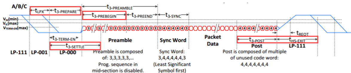
C-PHY High-Speed Data Transmission in Burst
