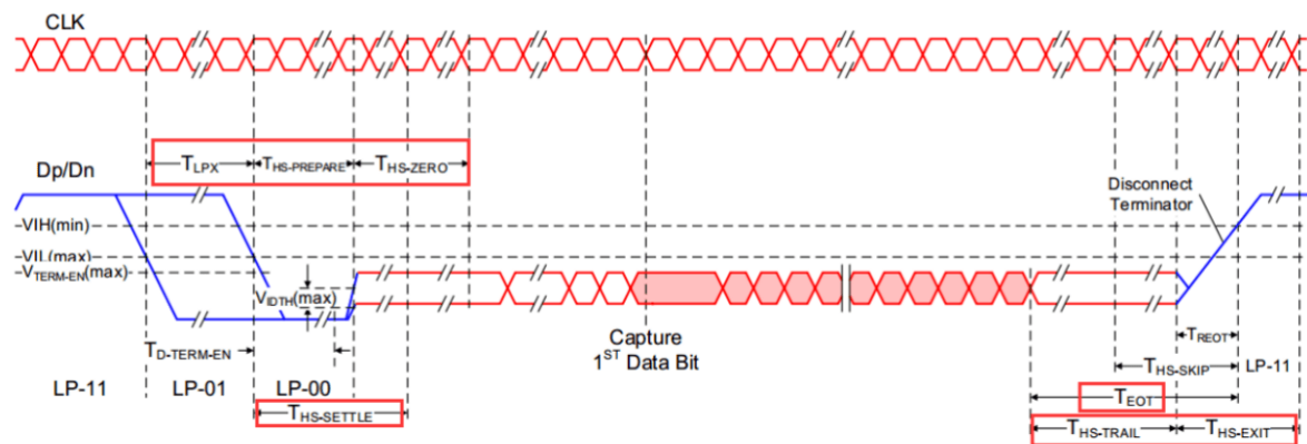
D-PHY High-Speed Data Transmission in Burst
