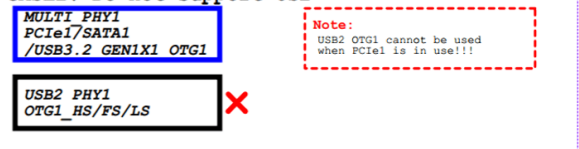
图 4 RK3576 OTG1 MULTI PHY Path Map
